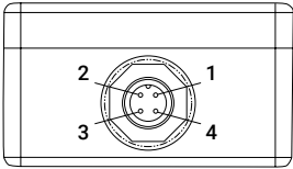
Connection plug arrangement (M12x1 / 4-pole round connector)
