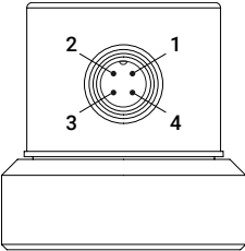
Connection plug arrangement (M12x1 metal / 4-pole round connector)
