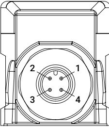
Connection plug arrangement (M12x1 metal / 4-pole round connector)
