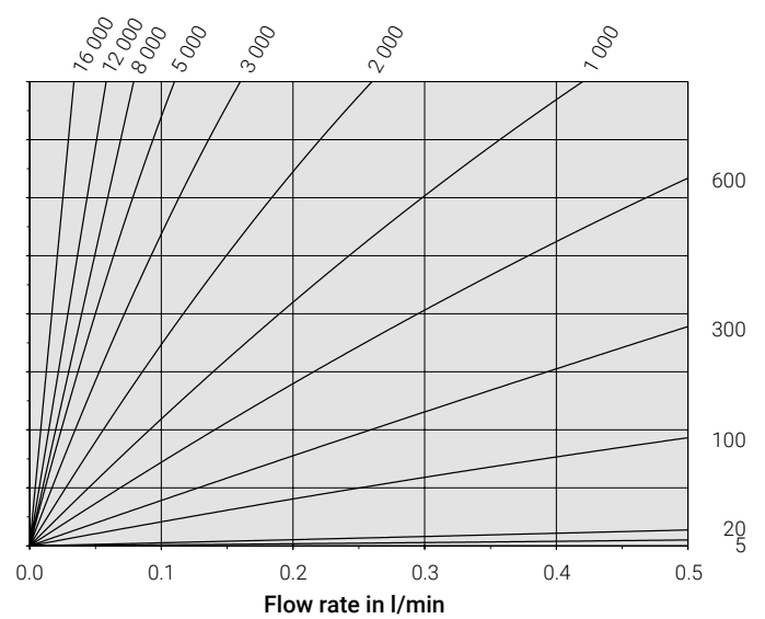
VC 0.1 (section)
