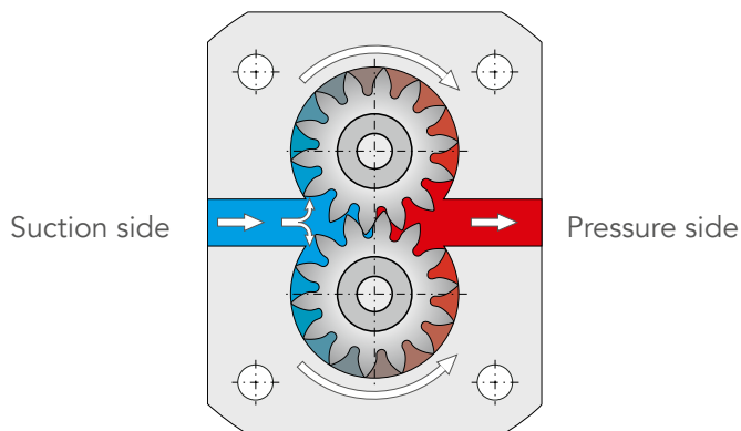
Suction side Pressure side Pump clockwise running
