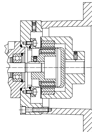
Pump with magnetic coupling
