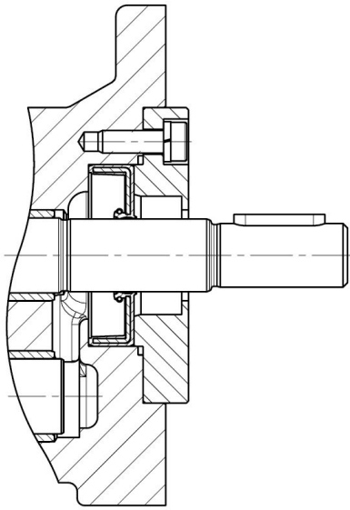
Rotary shaft seal Special number 100 Seal type : 2; 32
