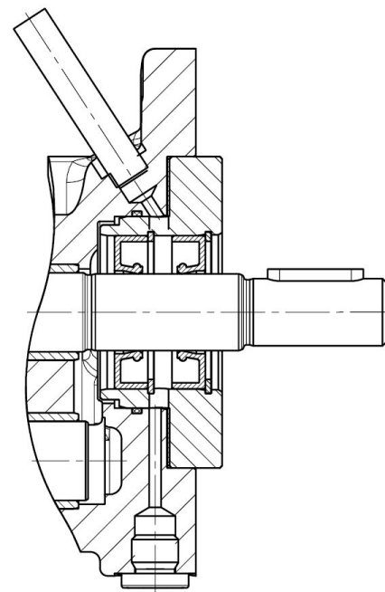
Rotary shaft seal (for vacuum operation) Connecting pipe 8x1 (for fluid buffer) Special number 242 Seal type : 2
