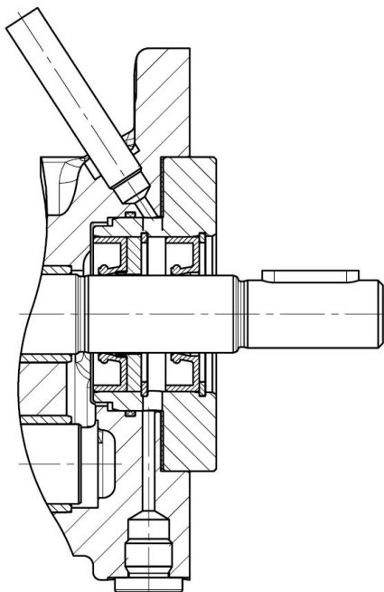
Double rotary shaft seal Connecting pipe 8x1 (for fluid buffer) Special number : 130; 162; 223; 224; 294; 323 Seal type : 2; 32
