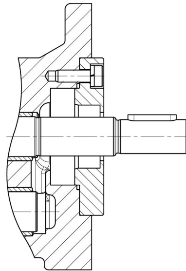
Without Shaft seal (Leak oil drain through shaft sealing chamber ) Special number : 456 Seal type : 61
