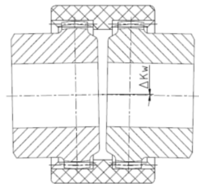
Angular displacement \Delta K_w
