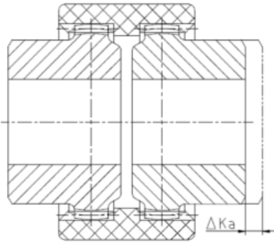
Axial displacement \Delta K_a
