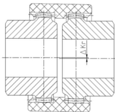
Radial displacement \Delta K_r
