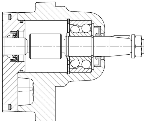
Rotary shaft seal with Outbord bearing , heavy-duty version Seal type : 1; 2
