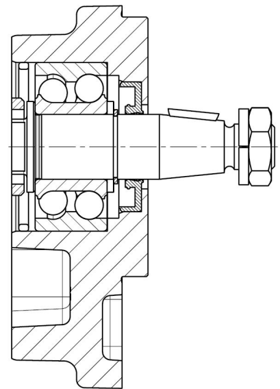
Rotary shaft seal with Outbord bearing Light-duty design Seal type : 1; 2
